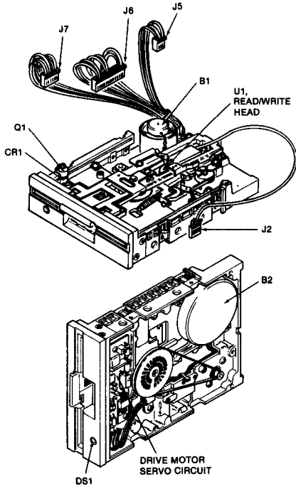
Fig. A-20. Drive unit parts layout, Model 1540.
